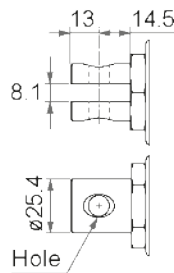
2 : Metal slot, hole \varnothing 12.2mm 4 : Metal slot, hole \varnothing 13mm
