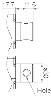
1 : Metal solid, hole \varnothing 12.2mm 3 : Metal solid, hole \varnothing 13mm
