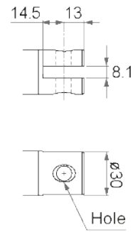
6 : SUS304 slot, hole \varnothing 12.2mm 8 : SUS304 slot, hole \varnothing 13mm
