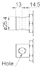
1 : Metal solid, hole \varnothing 12.2mm 3 : Metal solid, hole \varnothing 13mm
