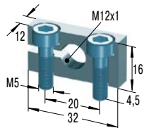
MB12 Klemflens
