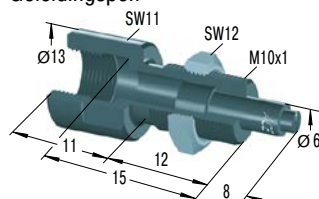
BV10SC Geleidingspen
